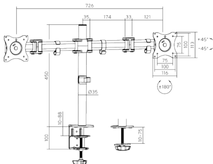
Dimensions (mm)
